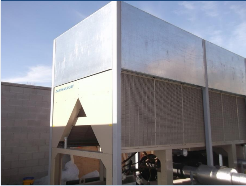
Finished UnitaryPlus™ “IS” System Acoustical Discharge Stack
