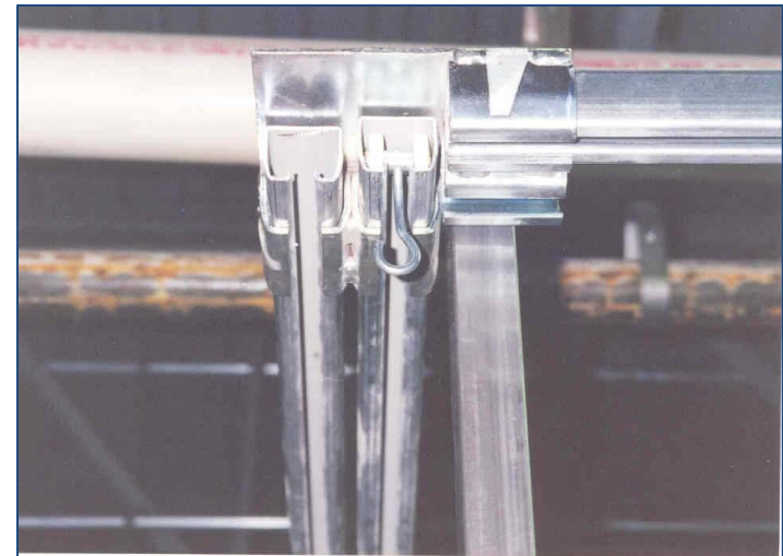
Close-Up of Double Track Galvanized Steel Framework and Sliding Roller Trolleys
