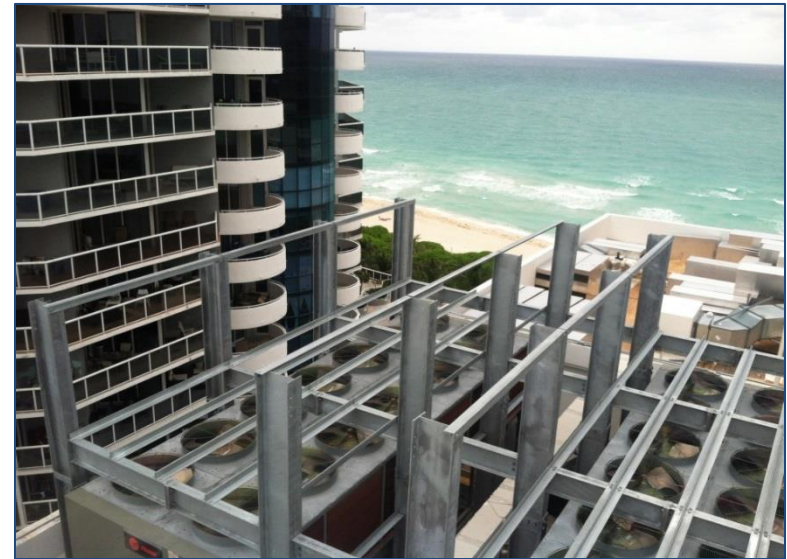
Completed Steel Framing PE Stamped for Hurricane Wind Load
