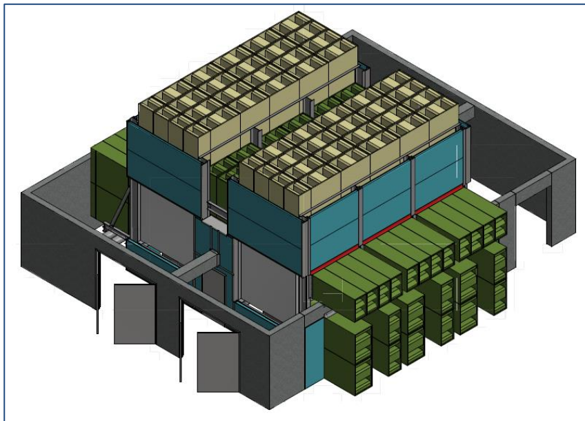
Northeast Isometric View
