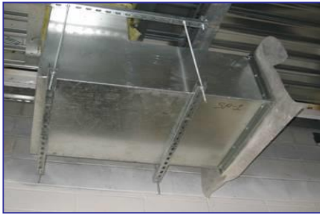
Plenum Style Curb & HUSH DUCT™ Elbow Silencer
