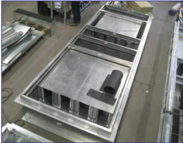
Top view of completed ULTRA ™ System
